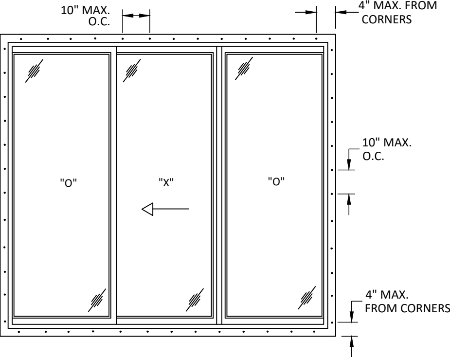
TYPICAL ANCHOR LAYOUT NAIL FIN INSTALLATION
