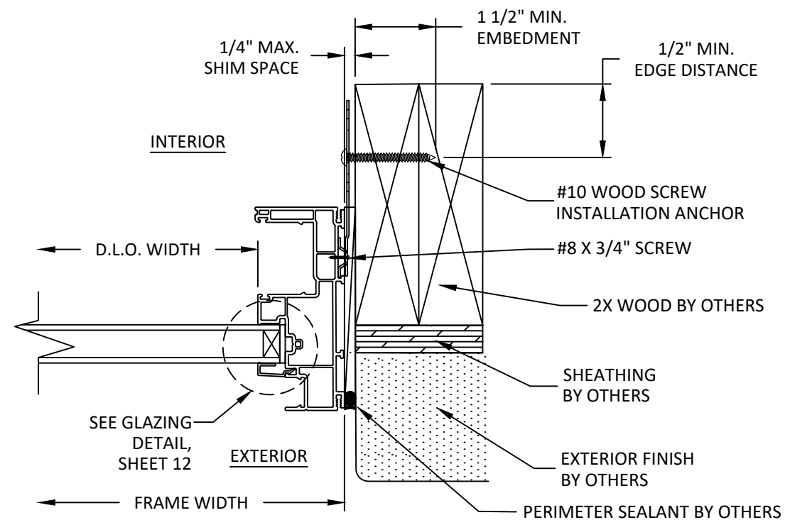
B 11 HORIZONTAL SECTION CLIP INSTALLATION WOOD SUBSTRATE
