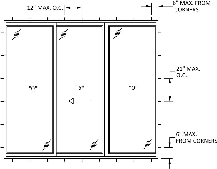
TYPICAL ANCHOR LAYOUT THROUGH FRAME/CLIP INSTALLATION
