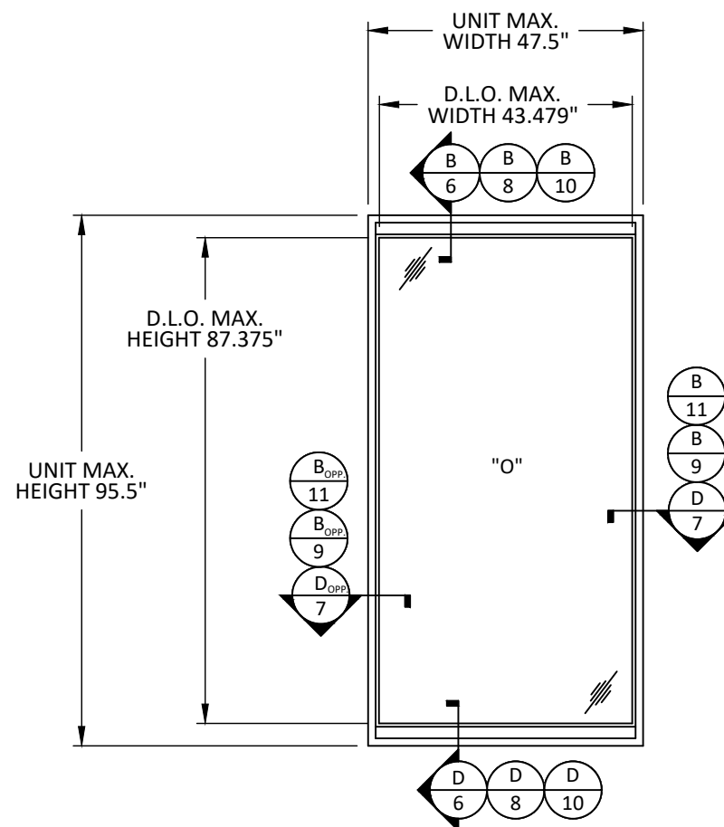
TYPICAL ELEVATION
