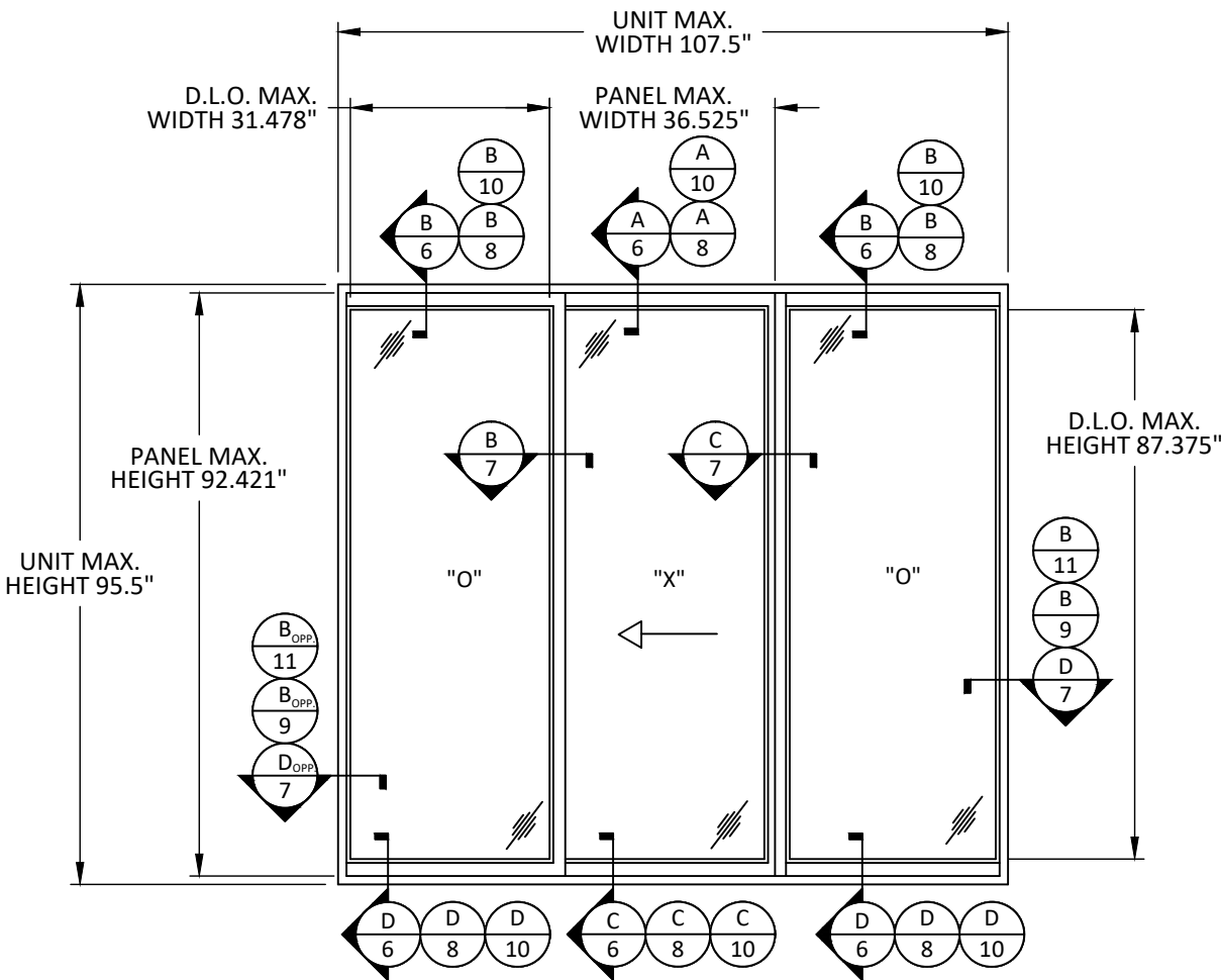
TYPICAL ELEVATION
