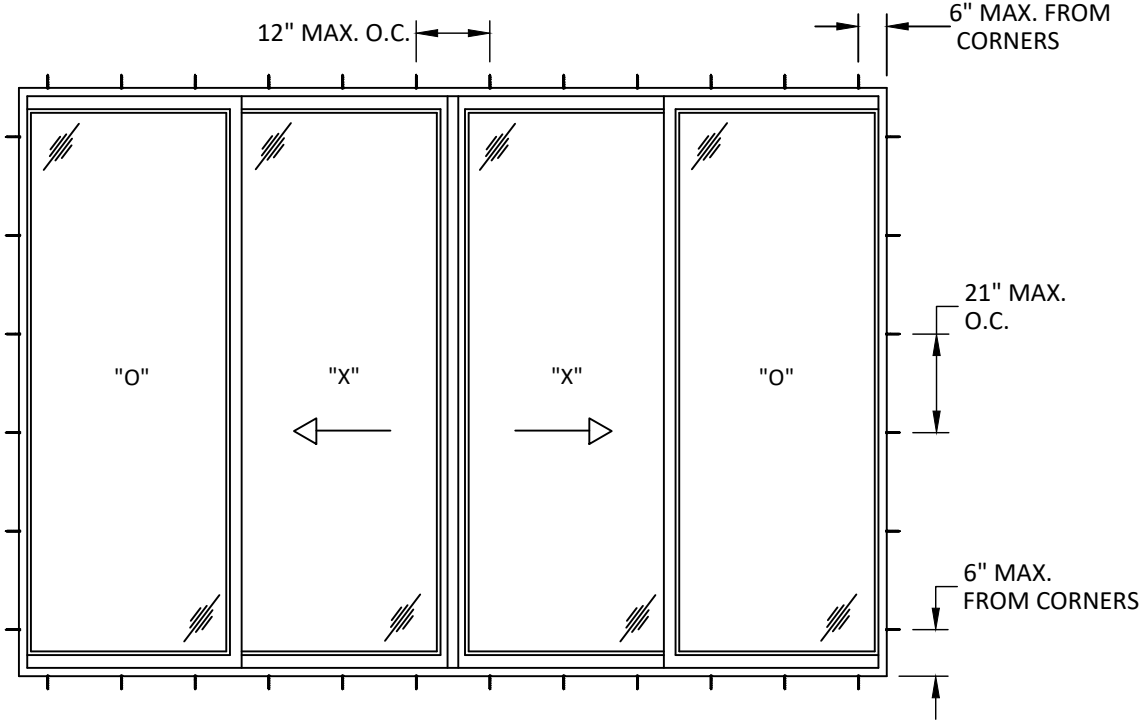
TYPICAL ANCHOR LAYOUT THROUGH FRAME/CLIP INSTALLATION
