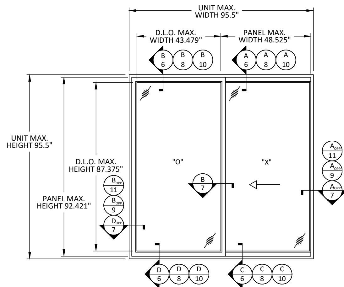
TYPICAL ELEVATION
