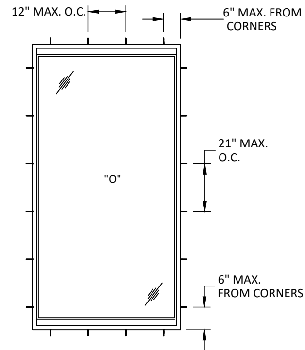
TYPICAL ANCHOR LAYOUT THROUGH FRAME/CLIP INSTALLATION
