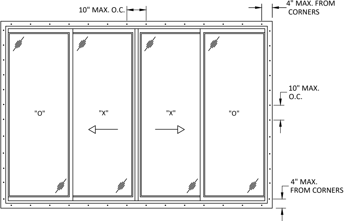
TYPICAL ANCHOR LAYOUT NAIL FIN INSTALLATION
